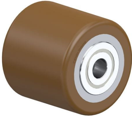
Corresponding caster (Ball bearing) HB 85x80/17-82K
